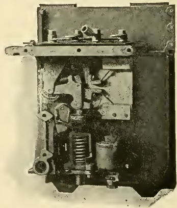
Fig. 68. View of Westinghouse Unit Switch
